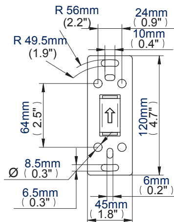
Wall Plate
