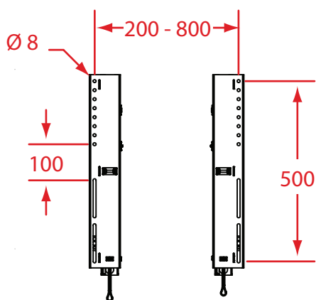
PANEL ATTACHMENT - VESA COMPATABILITY (mm)
