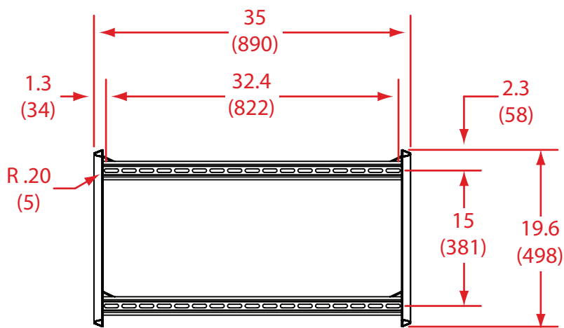
WALL MOUNTING
