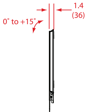
MOUNTING PROFILE
